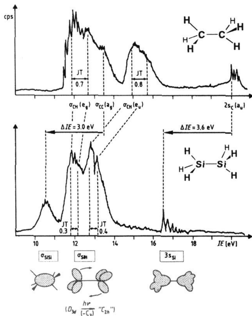
Figure 4. Comparison of the He I PE spectra of ethane and disilane, exhibiting Jahn/Teller splitting ( J/T ) of their M^+ ( e ) states with predominant contributions ( \square ) to positive hole delocalization (cf. the text).
