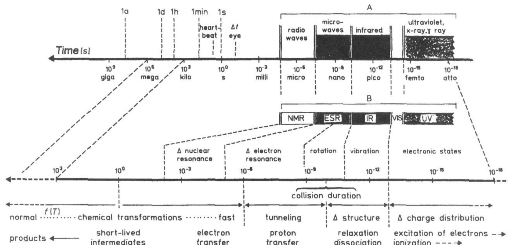
Figure 3. Schematic time scale for molecular states and their changes (in seconds).
