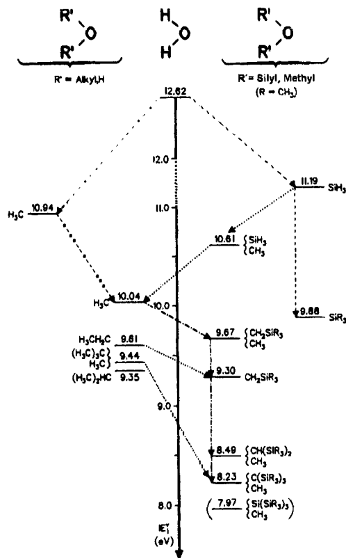
Figure 15. First vertical ionization energies IE_1^v(nO) (eV) of H_2O and its alkyl, silyl, trimethyl, and (trimethylsilyl)-methyl derivatives: (---) identical mono- and disubstitution, (· ·) alkyl/silyl comparison, and (— · —) \beta -silyl substituent effects.
