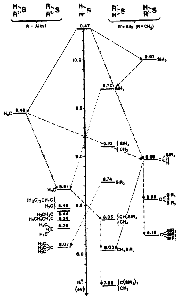
Figure 14. First vertical ionization energies IE_1^v(ns) (eV) of H_2S and its alkyl, silyl, trimethyl and (trimethylsilyl)-methyl derivatives: (---) identical mono- and disubstitution, (· ·) alkyl/silyl comparison, (— · —) \beta -silyl substituent effects.
