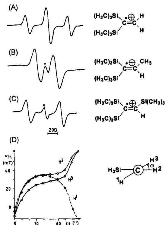
Figure 22. ESR spectra of organosilicon radical cations generated in trichlorofluoromethane matrices at 77 K by 60 Co \gamma -irradiation: (A) 1,1-bis(trimethylsilyl)ethylene, (B) 1,1-bis(trimethylsilyl)-2-methylethylene, and (C) 1,1,2-tris(trimethylsilyl)ethylene (X, signals from unidentified species; cf. the text). (D) INDO open shell hypersurface for the dependence of the coupling constants a_{\text{H}} on the dihedral angle ( \omega ) in vinylsilane.
