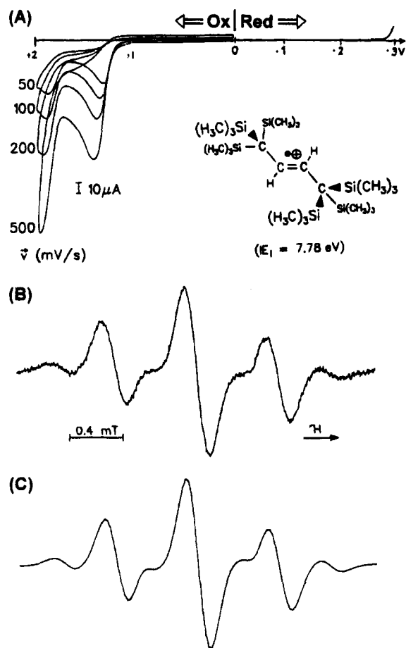
Figure 24. 1,1,1,4,4,4-Hexakis(trimethylsilyl)-2-butene ( \text{IE}_1^{\text{v}} = 7.78 \text{ eV} ): 62 (A) cyclic voltammograms for oxidation ( \text{H}_2\text{CCl}_2/0.1 \text{ M R}_4\text{N}^+\text{ClO}_4^- , GCE vs SCE) and reduction between 0 and -3 V ( v = 100 \text{ mV/s} ), (B) ESR signal pattern of its radical cation generated with \text{SbCl}_5 in \text{H}_2\text{CCl}_2 , and (C) optimized simulation with the trial-and-error fitting coupling constants a_{\text{H}}(\text{CH}) = 0.606 \text{ mT} , a_{\text{H}}(\text{CH}_3) = 0.022 \text{ mT} , and a_{^{29}\text{Si}} = 0.767 for 2, 54, and 6 equivalent centers, respectively (see the text).
