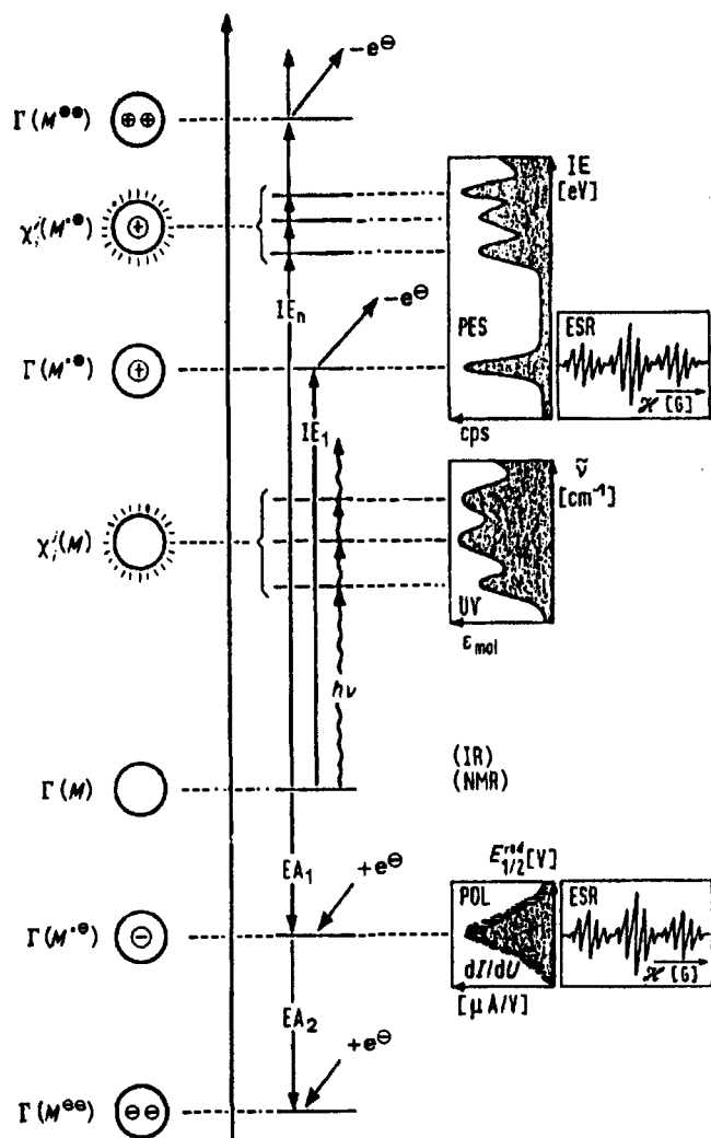
Figure 2. Schematic energy scale for electronic ground ( \Gamma ) and excited ( \chi_j ) states of a neutral molecule M , its radical cation M^{\bullet+} or dication M^{2+} generated by ionization or oxidation and its radical anion M^{\bullet-} and dianion M^{2-} resulting from electron insertion. Representative measurement methods used in many investigations are NMR, IR, UV, PE, ESR, and ENDOR spectroscopy as well as polarography (POL) or cyclic voltammetry.
