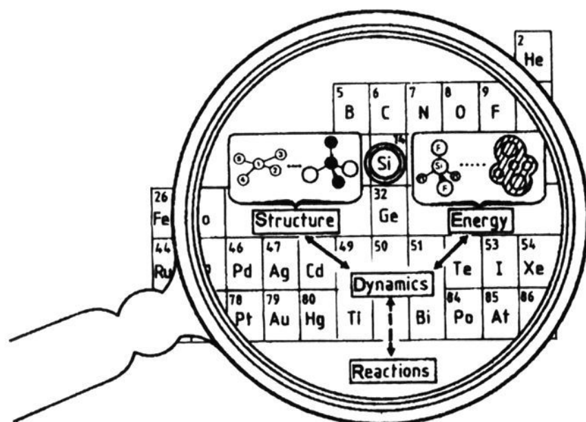
Figure 1. "Molecular-state magnifying glass" for the silicon chemist.
