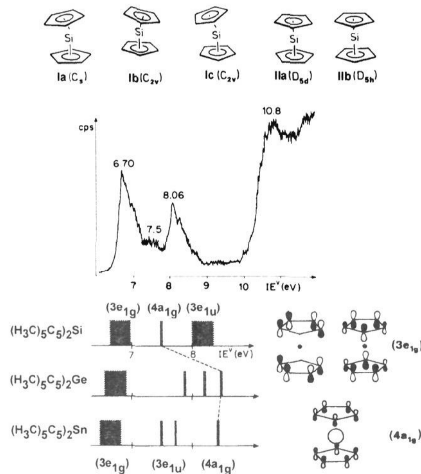
Figure 18. He I PE spectrum (6–10 eV) of bis( \eta^5 -pentamethylcyclopentadienyl)silicon as the most likely conformer Ia (cf. the text) and its assignment by both Koopmans' correlations, IE_n^v = \epsilon_j^{MND0} , as well as by radical cation state comparison with its Ge and Sn analogues (cf. the text).
