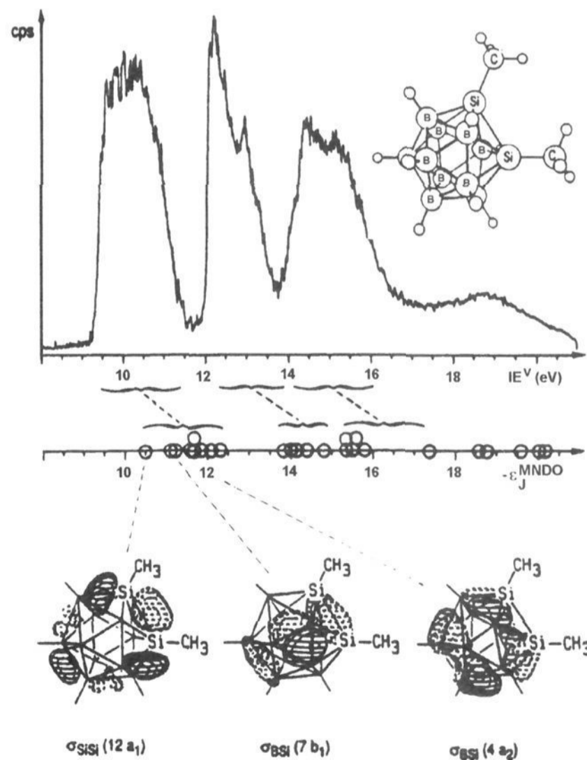
Figure 19. He I PE spectrum of 1,2-dimethyl-1,2-disila- closo -dodecaborane(12) ( (H_3CSi)_2B_{10}H_{10} ) with Koopmans' assignment by MND0 eigenvalues and cluster orbital diagrams for the three radical cation states of lowest energy.
