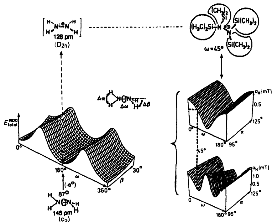
Figure 11. INDO open shell hypersurfaces both for the total energy and the structure of the radical cation \text{H}_2\text{NNH}_2^{+\bullet} as well as for the angular dependence of the coupling constants \alpha_N and \alpha_H including a structural estimate for the sterically overcrowded tetrakis(trimethylsilyl)hydrazine radical cation in solution (cf. the text).
