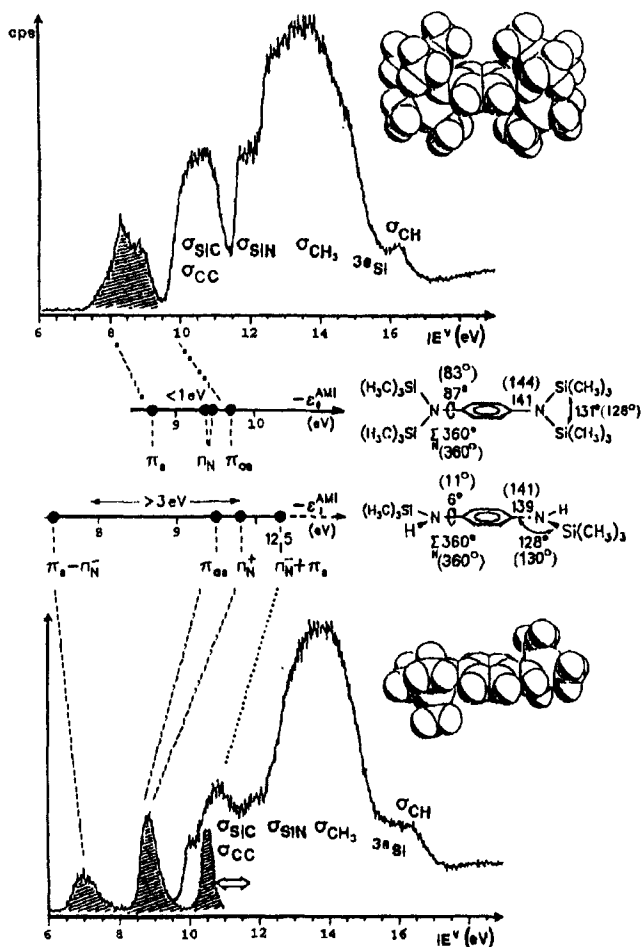
Figure 16. He I photoelectron spectra (6–18 eV) of N,N' -bis(trimethylsilyl)- and N,N,N',N' -tetrakis(trimethylsilyl)- p -phenylenediamines with Koopmans' assignment, IE_n = -\epsilon_j^{AM1} , based on the eigenvalues of geometry-optimized AM1 calculations, the structural data of which are given. Also shown are space-filling representations of the single crystal structures carried out for the neutral molecules (values in brackets; cf. the text).
